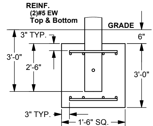
FOOTING DETAIL
