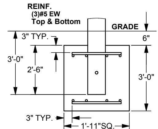
FOOTING DETAIL
