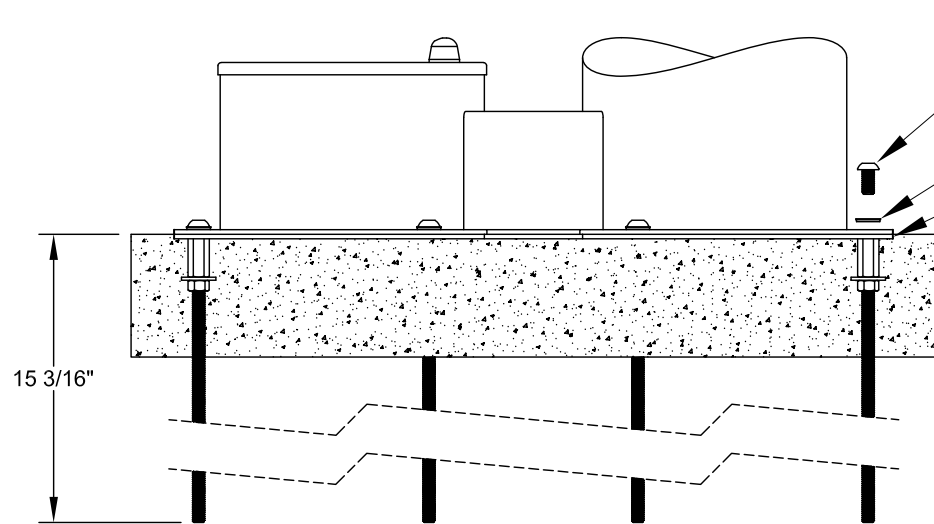
TYPICAL INSTALLATION
