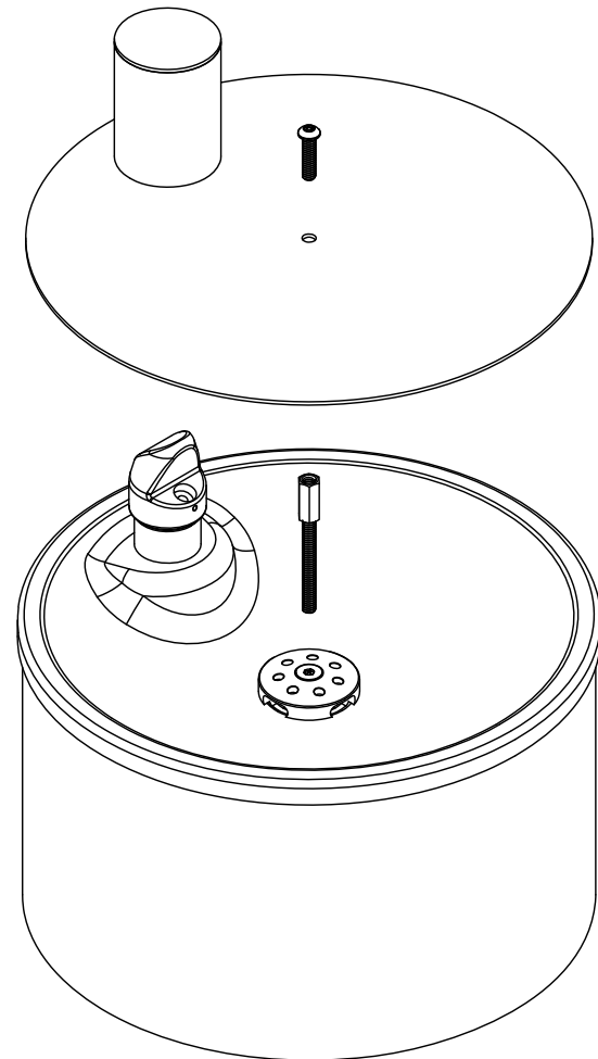
TYPICAL INSTALLATION
