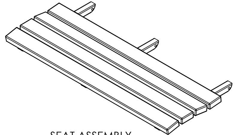
SEAT ASSEMBLY ABC-A0023 X1
