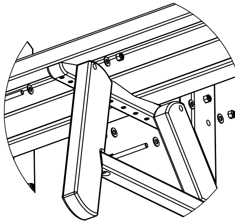
Underside Detail View
