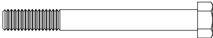
3/8-16 X 3.5" HEX HEAD BOLT X20 F0001
