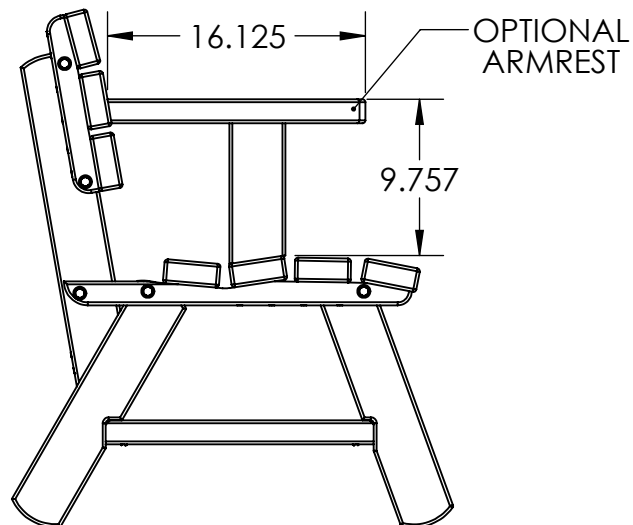
③ BENCH WITH ARMREST DETAILS
