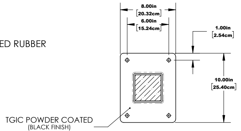
MOUNTING DETAILS
